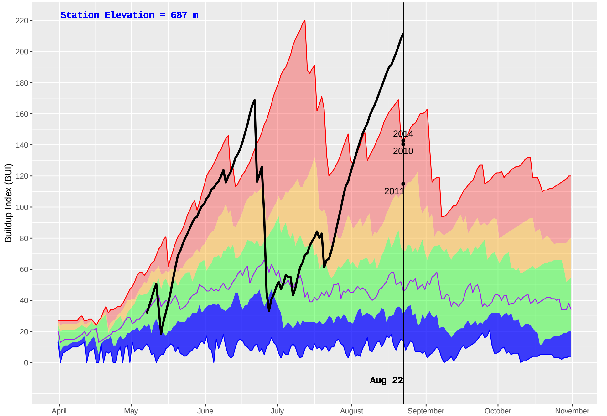
KETCHIKA (444) : Historical (1986–2016) and Current (2018) Daily Buildup Index (BUI)
